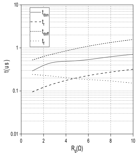
开关时间 IGBT, 逆变器 (典型值) Switching time IGBT, Inverter (typical) t = f(R_G) I_C = 450A, V_{CE} = 600V, V_{GE} = 15V/-8V T_{vj} = 175^\circ C
