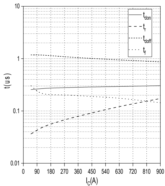
开关时间 IGBT, 逆变器 (典型值) Switching time IGBT, Inverter (typical) t = f(I_C) R_{Goff} = 5.1\Omega, R_{Gon} = 1.0\Omega, V_{CE} = 600V V_{GE} = 15V/-8V, T_{vj} = 175^\circ C
