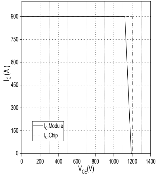
反偏安全工作区 IGBT, 逆变器(RBSOA) Reverse bias safe operating area IGBT, Inverter (RBSOA) I_C = f(V_{CE}) , V_{GE} = 15V/-8V, R_{Goff} = 5.1\Omega, T_{vj} = 175^\circ C
