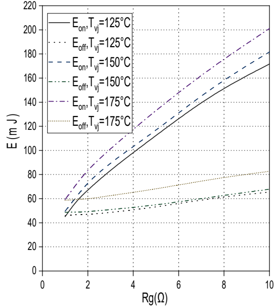
开关损耗 IGBT, 逆变器 (典型值) Switching losses IGBT, Inverter (typical) V_{GE} = 15V/-8V, I_C = 450A, V_{CE} = 600V
